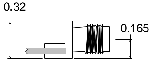
Connector detail, side view TYP 3 plcs.
